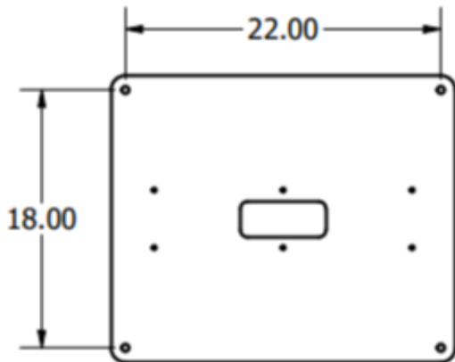
BASE PLATE MOUNTING DIMENSIONS
